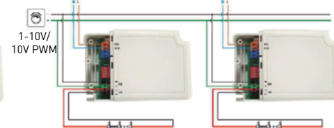
1-10V Regulation
